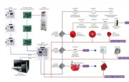
Addressable Fire Alarm System
